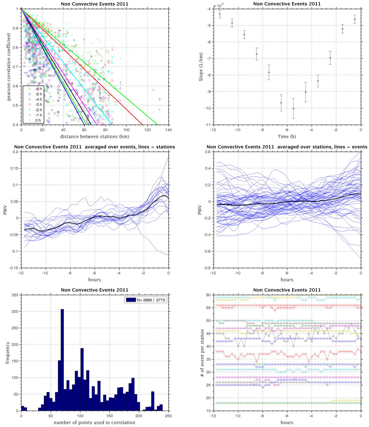
Figure 16: Non_Convective_Events_2011_12hr_interval_output.dat, ntimes=48, nevents=60, nstation=21, max dist=150
