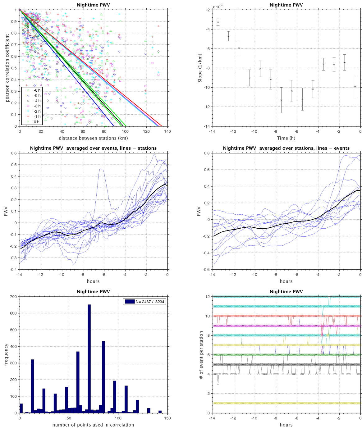
Figure 5: Nighttime_PWV_14hr_interval.2011_2012.dat, ntimes=168, nevents=12, nstation=21, max dist=150
