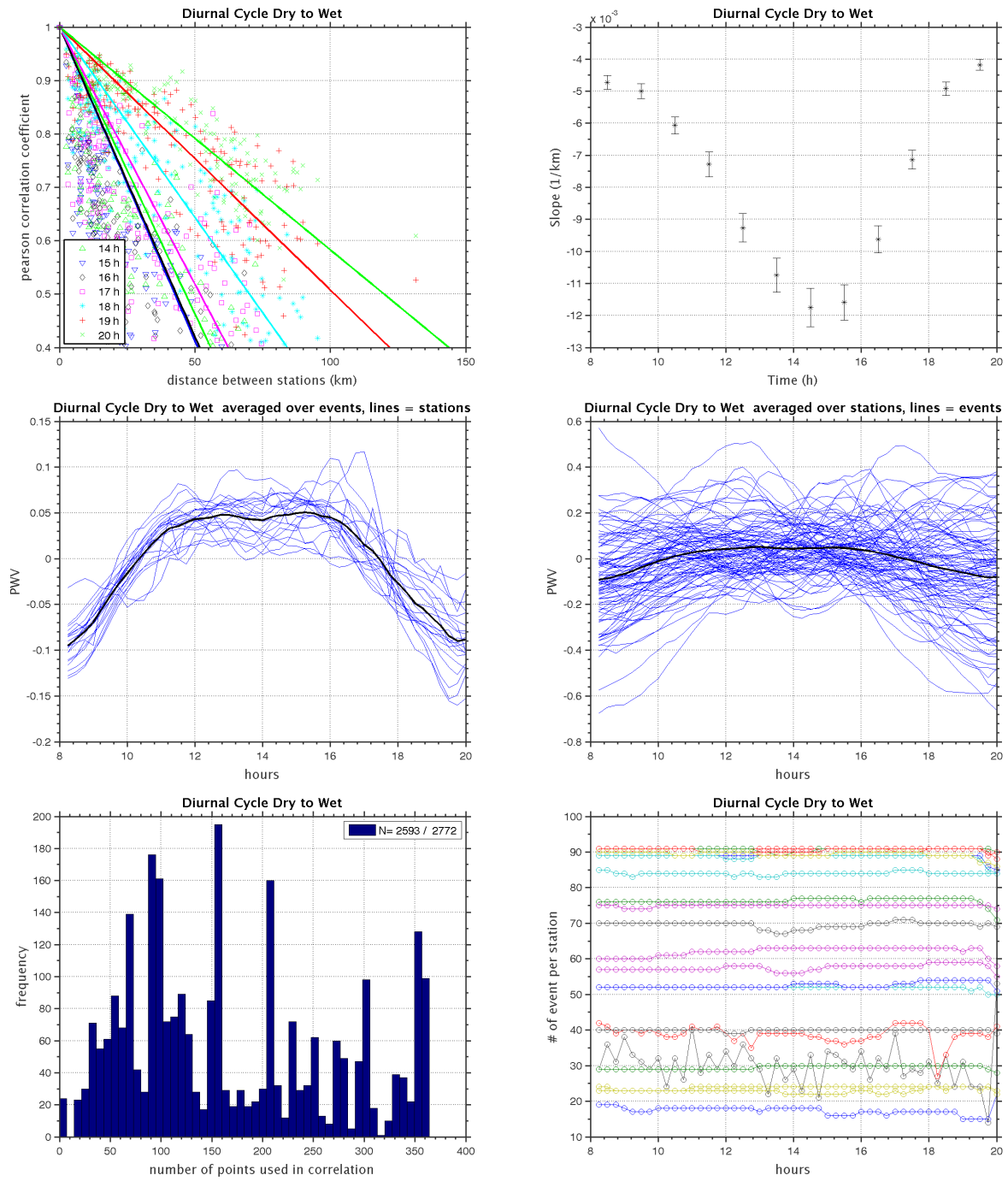
Figure 14: Diurnal_Cycle_Dry_to_Wet_12hr_interval.output.dat, ntimes=48, nevents=91, nstation=21, max dist=150
