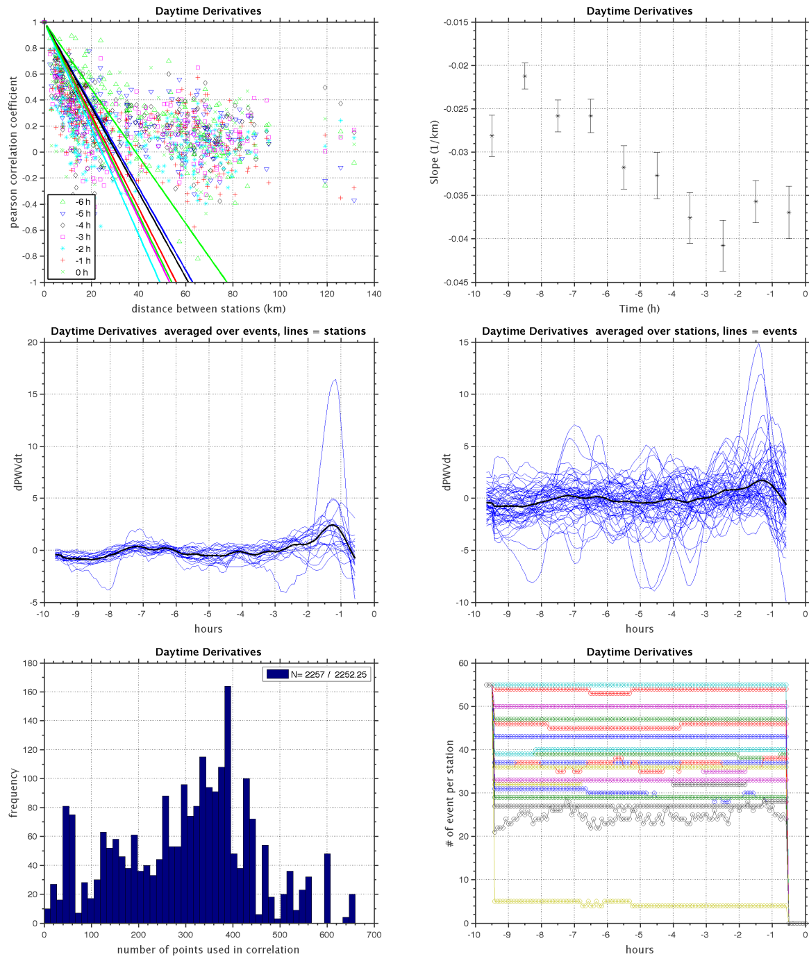
Figure 2: Daytime_Derivatives_9hr_interval_2011_2012.dat, ntimes=117, nevents=55, nstation=21, max dist=40
