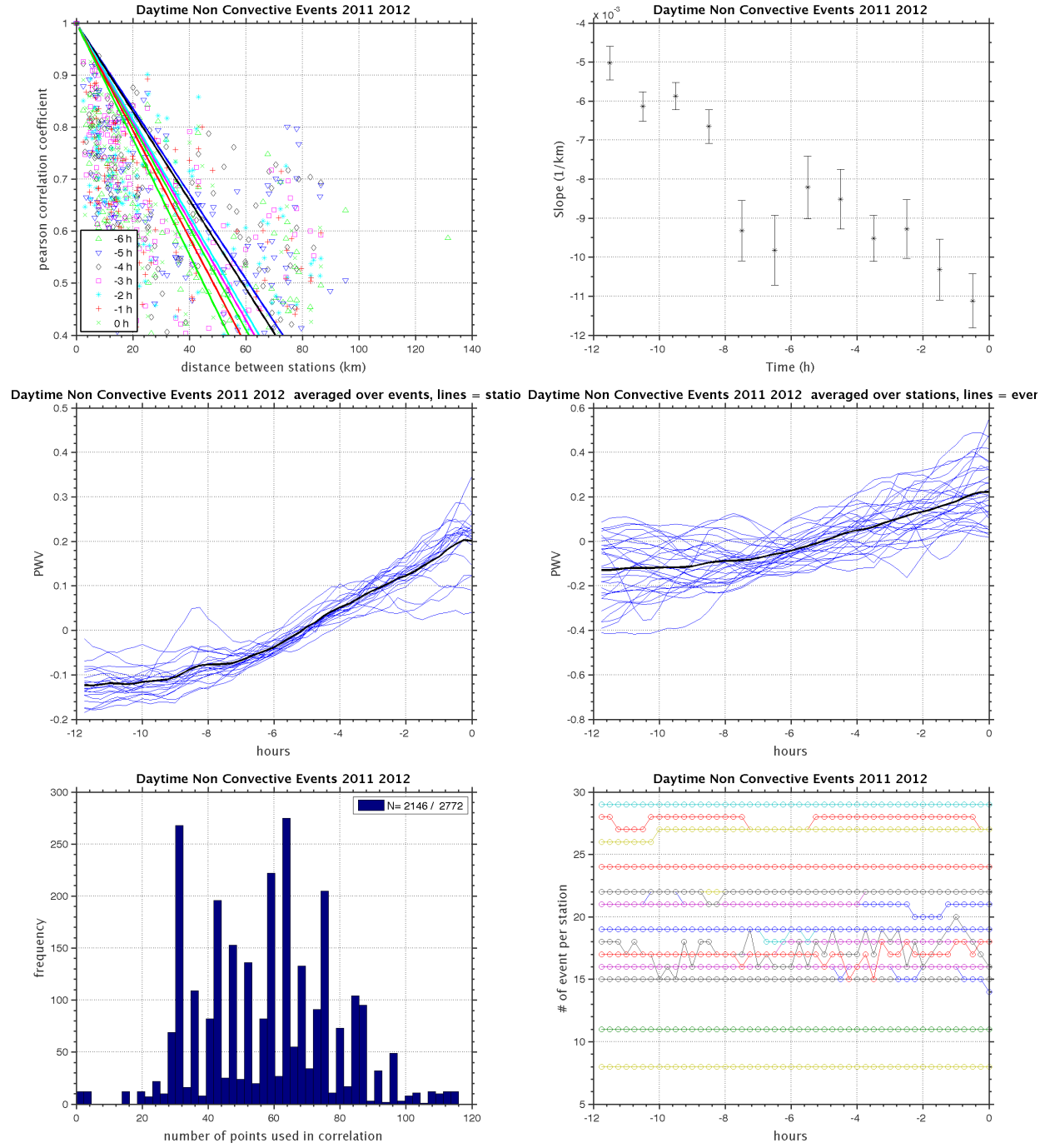
Figure 17: Daytime_Non_Convective_Events.2011.2012.12hr.interval.output.dat, ntimes=48, nevents=30, nstation=21, max dist=150
