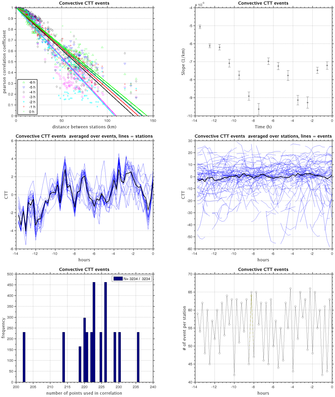
Figure 12: Convective_CTT_events.14hr_interval.output.dat, ntimes=56, nevents=69, nstation=21, max dist=150
