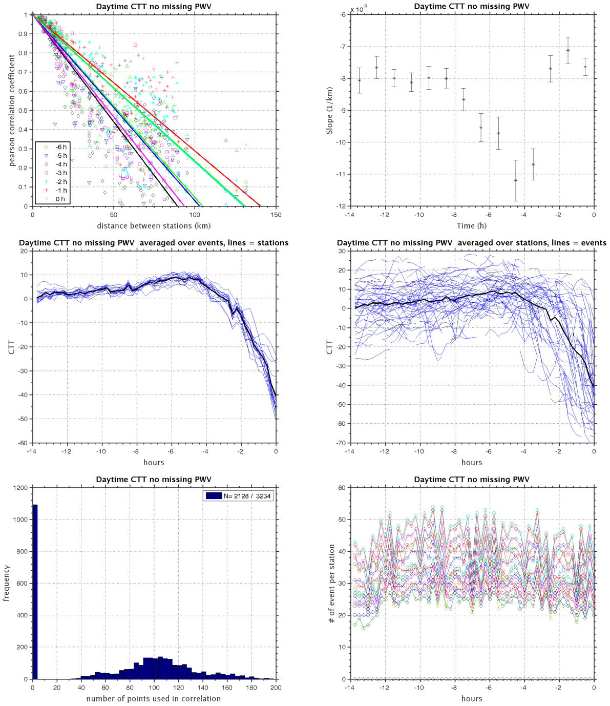
Figure 13: Daytime_CTT_no_missing_PWV_14hr_interval.2011.2012.dat, ntimes=56, nevents=55, nstation=21, max dist=150
