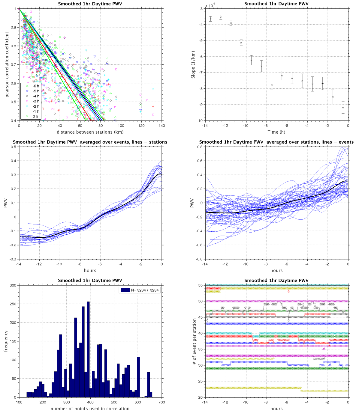
Figure 10: Smoothed_1hr_Daytime_PWV_14hr_interval_2011_2012.dat, ntimes=168, nevents=55, nstation=21, max dist=150
