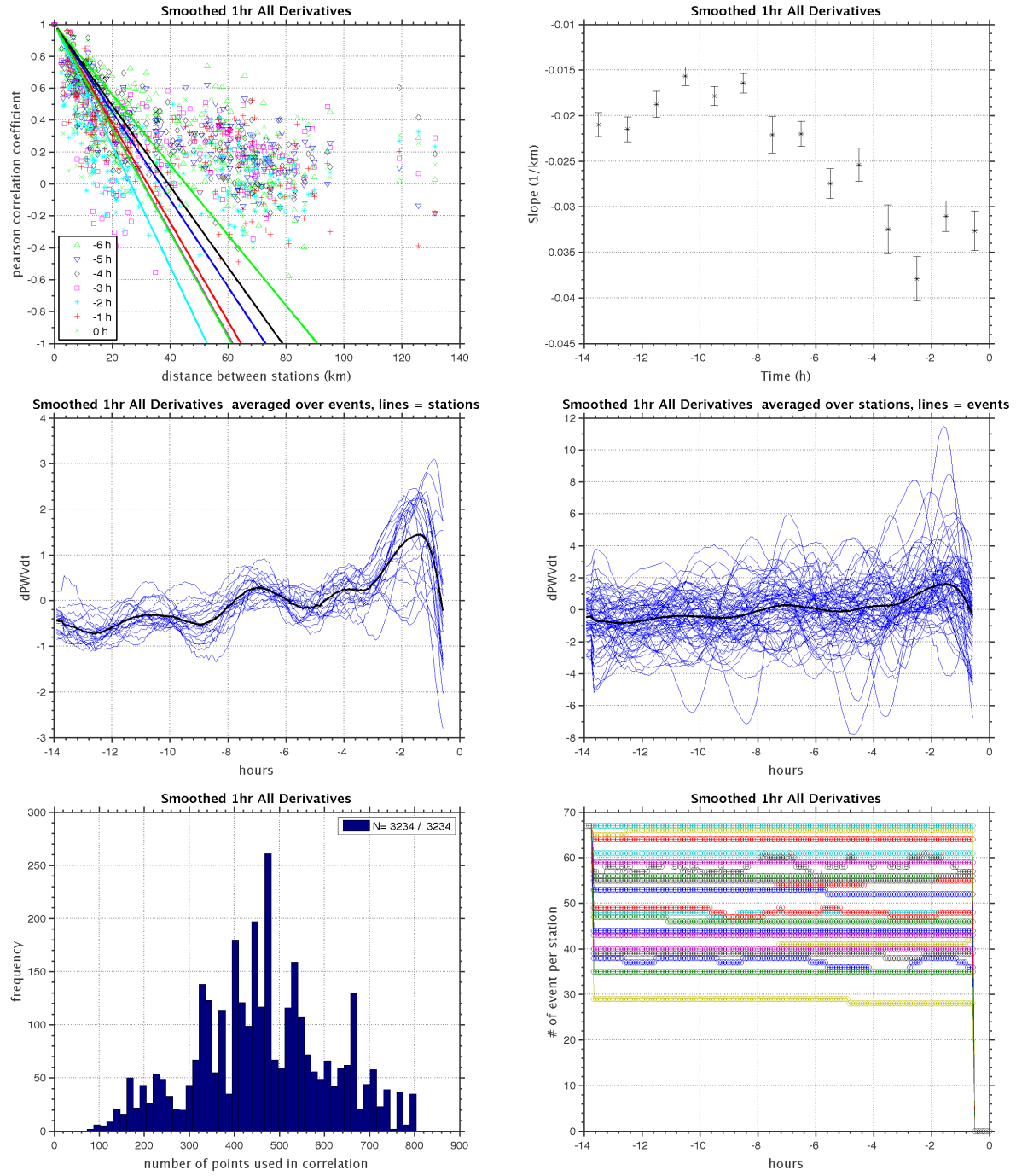
Figure 9: Smoothed_1hr_All_Derivatives_14hr_interval_2011.2012.dat, ntimes=168, nevents=67, nstation=21, max dist=40
