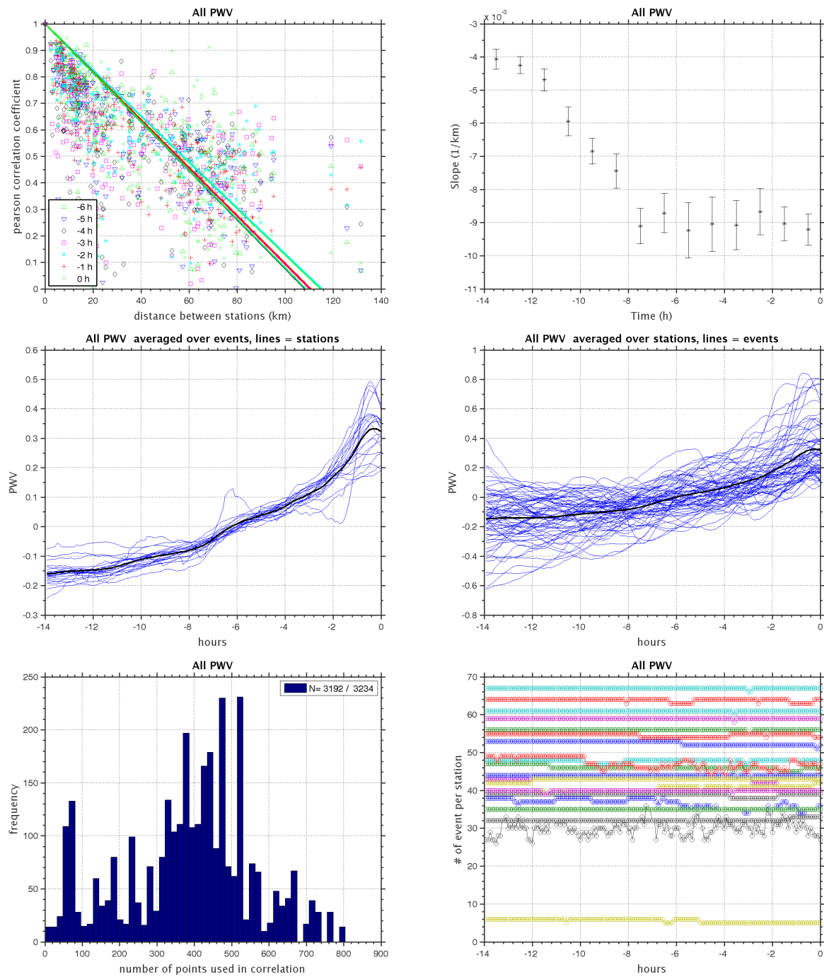
Figure 3: All_PWV_14hr_interval_2011_2012.dat, ntimes=168, nevents=67, nstation=21, max dist=150
