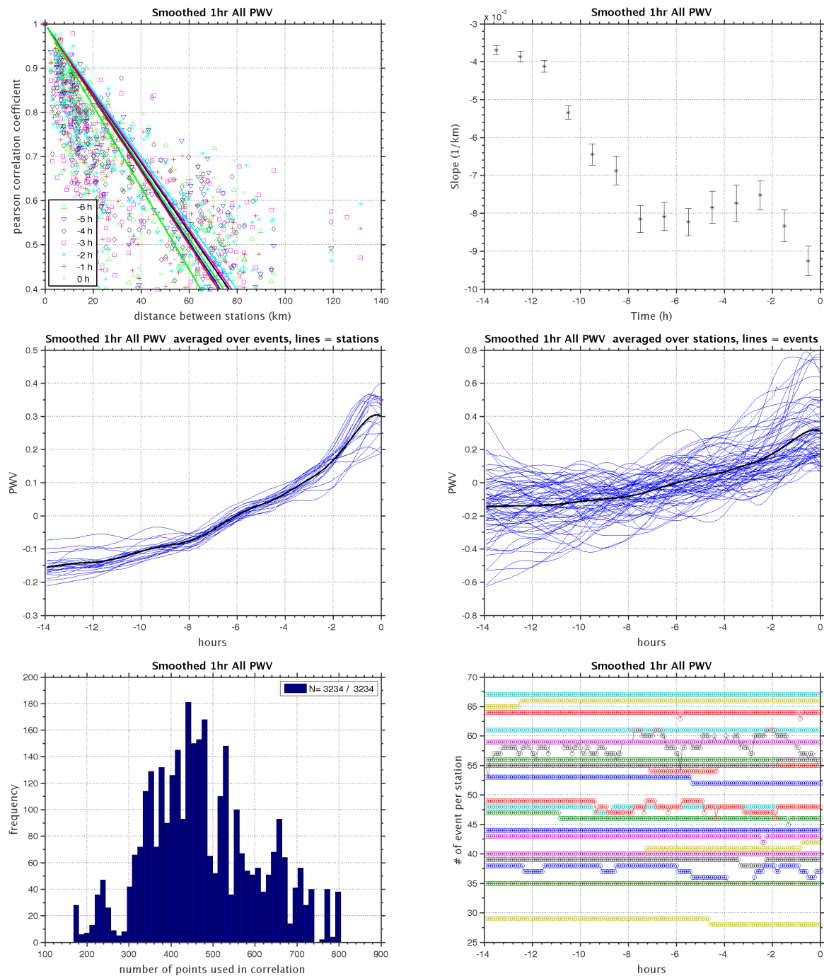
Figure 8: Smoothed_1hr_All_PWV_14hr_interval.2011.2012.dat, ntimes=168, nevents=67, nstation=21, max dist=150
